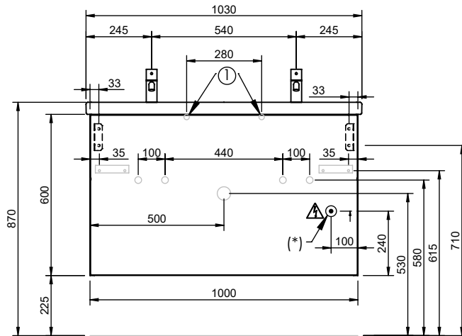
SFSR103 (*)SFSV103
